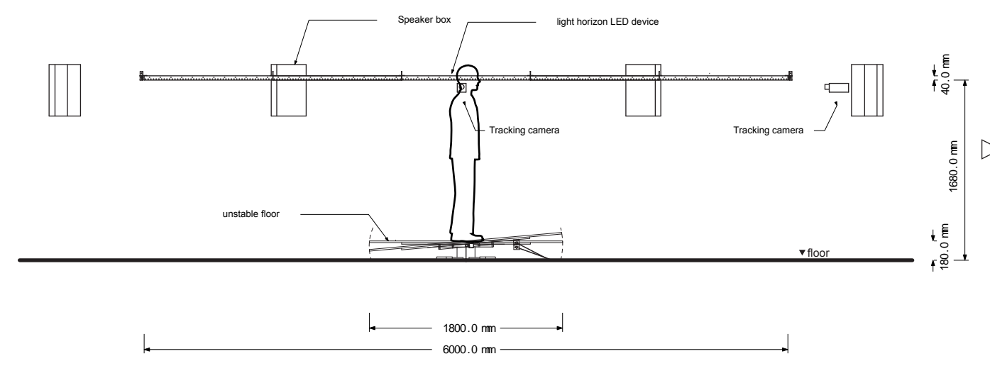
cross section 1/50
